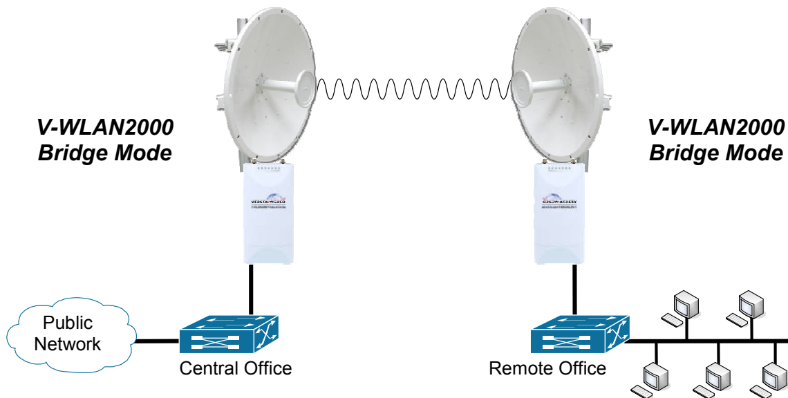
Figure 2-3: V-WLAN2000 Series as Wireless Bridge Mode Diagram
